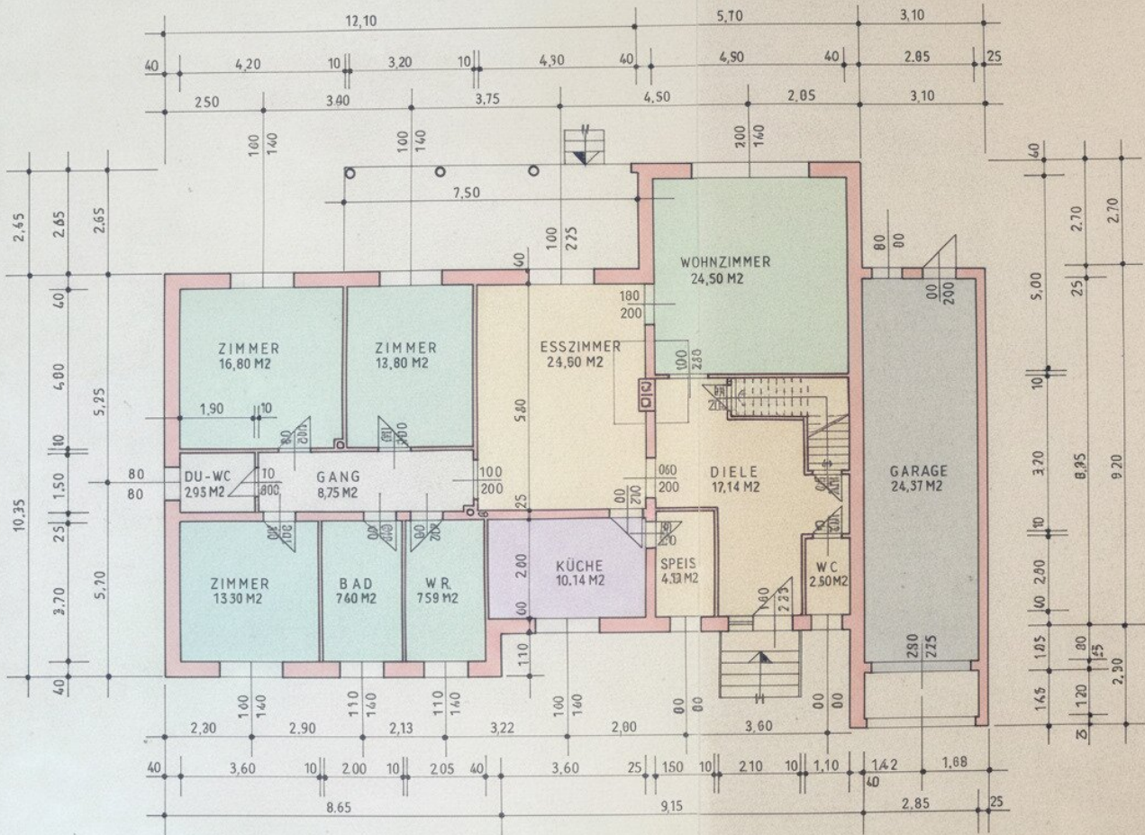
ERDGESCHOSS M = 1 : 100
