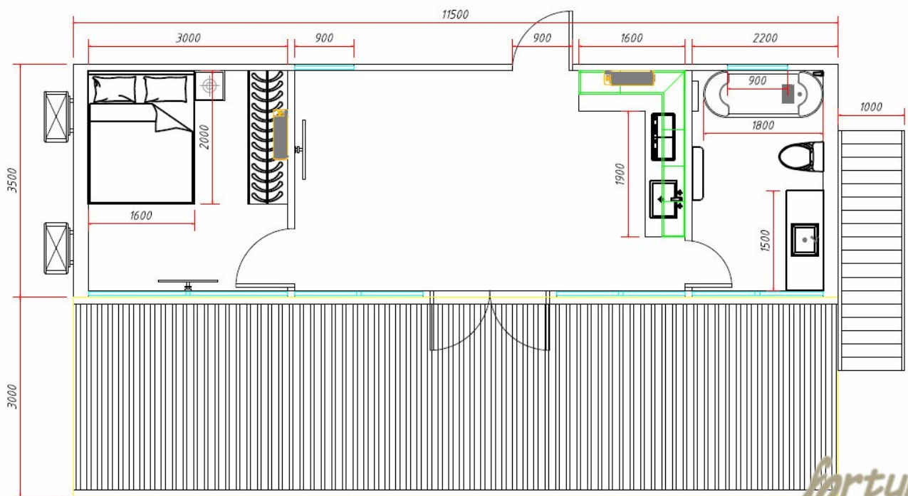
Floor Plan
