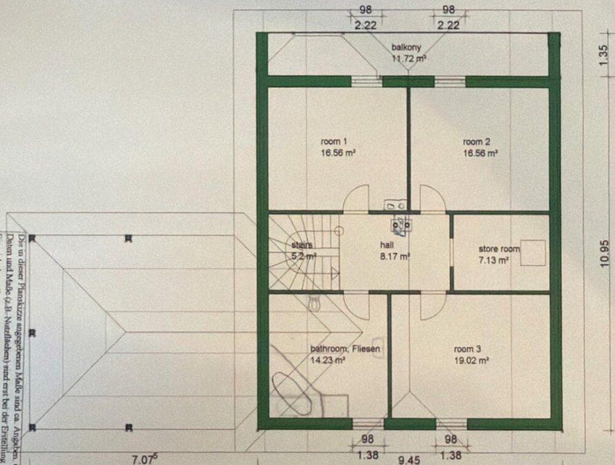
roof floor 86.88 sqm 1:100
