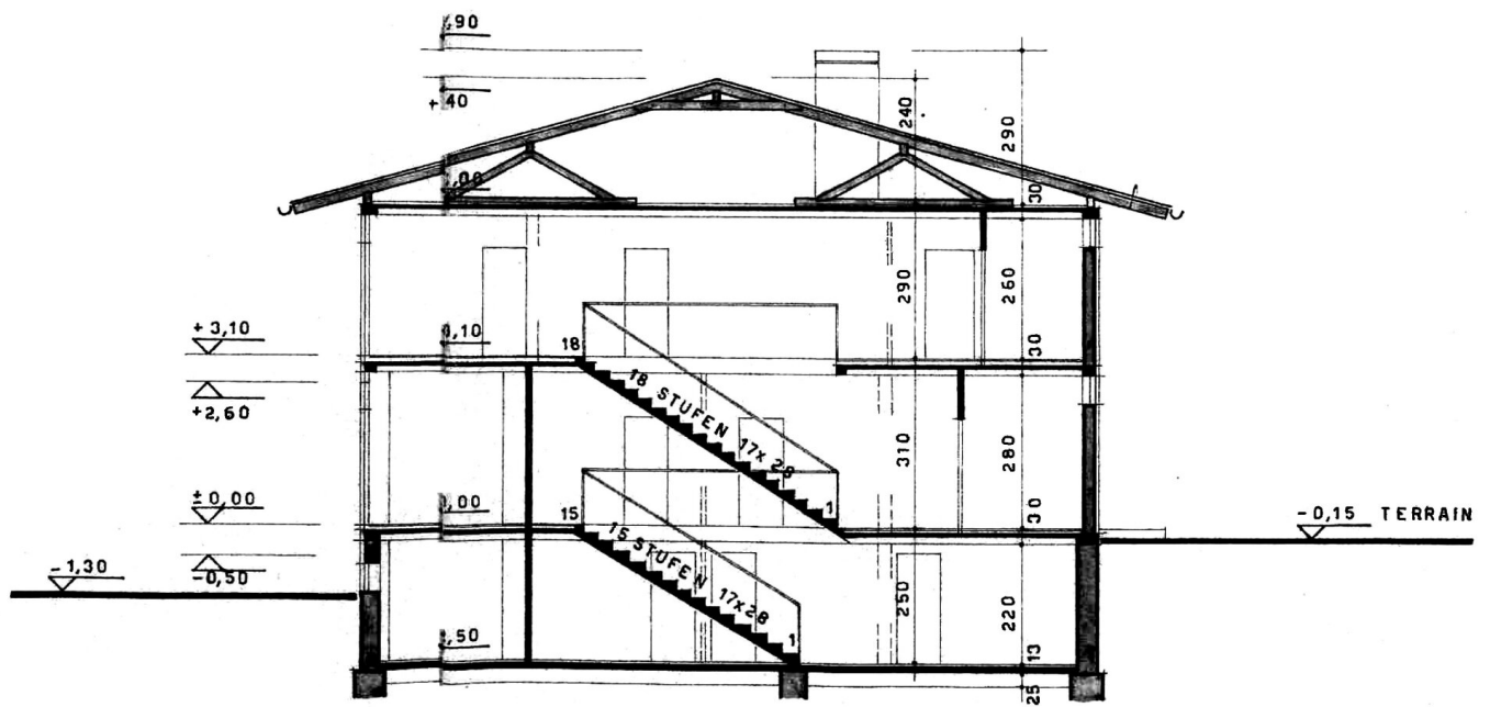
S C H N I T T 1 = 100
