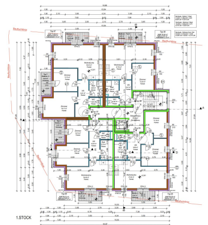
1. STOCK
