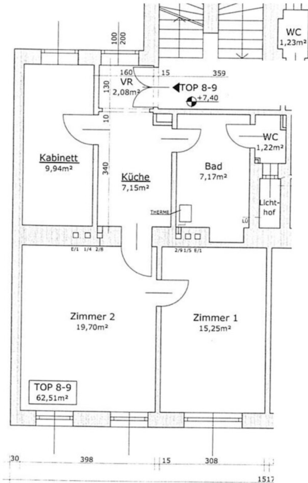
Grundriss 2. Stock
