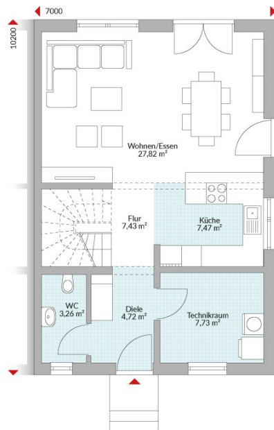
Erdgeschoss 58,43 m 2
