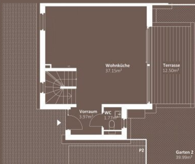
ERDGESCHOSS WNF 42,89m²
