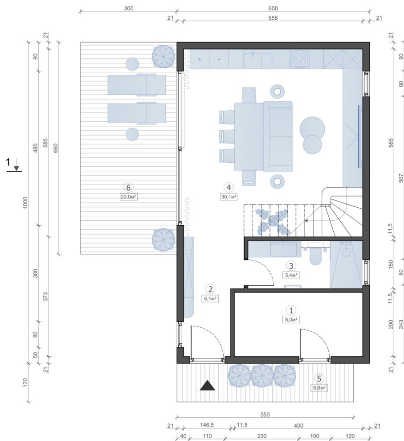
Erdgeschoss. M 1:50 (A-3)
