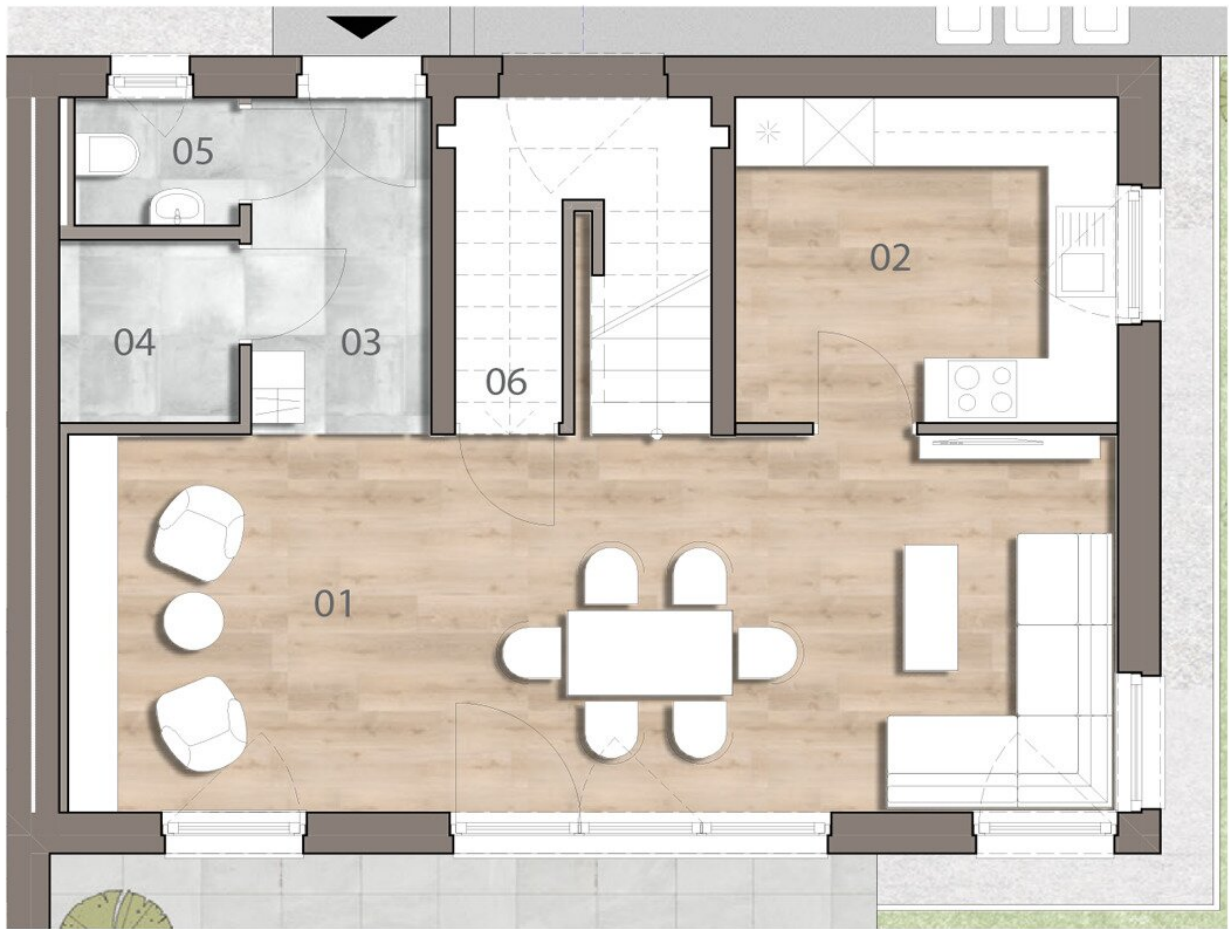
Erdgeschoss (optional)
