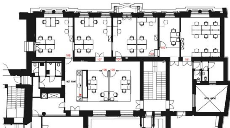
MEZZANINE LEVEL FLOOR PLAN (EXISTING)
