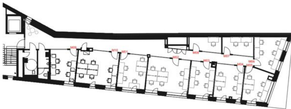
MEZZANINE LEVEL FLOOR PLAN (EXISTING)
